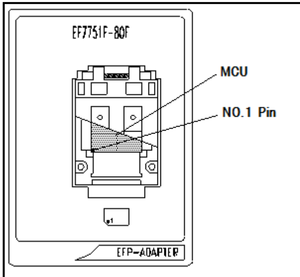
Fig.2.1 Insertion Direction of MCU
